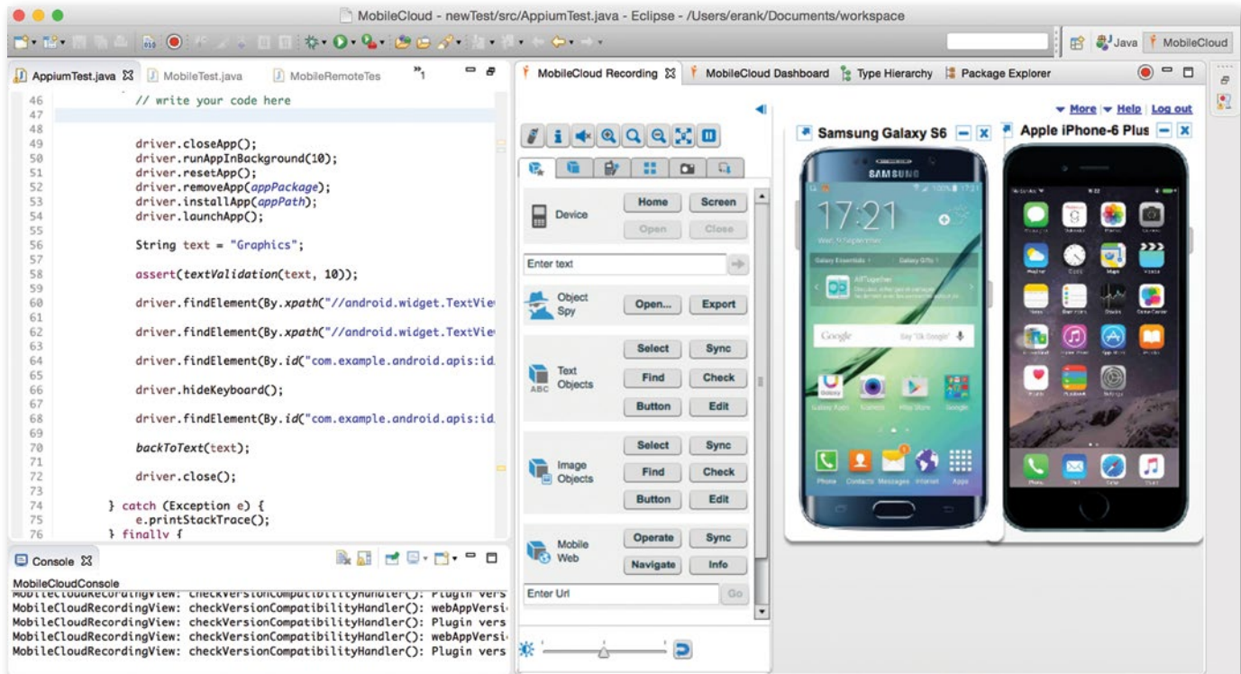
Cross-platform test automation using Appium on real devices.
